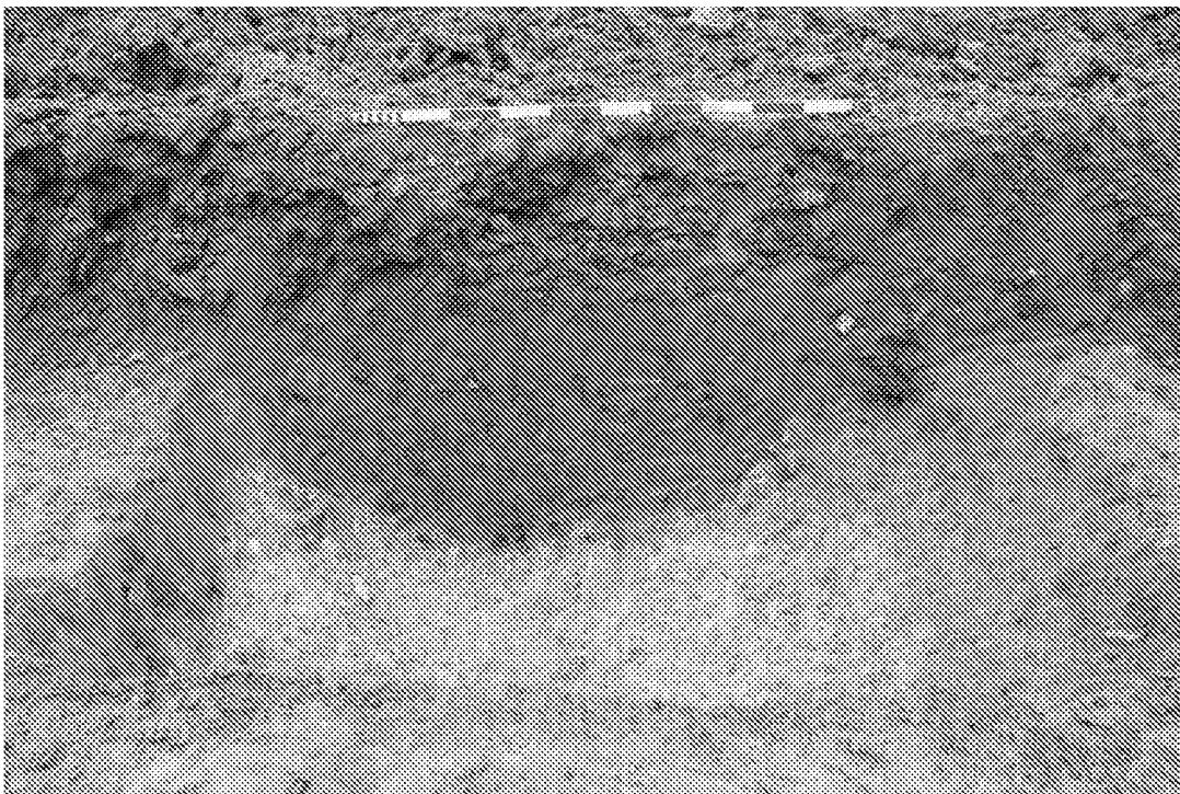
Plate 6. Section of ditch [404] view to east, scale 1m
