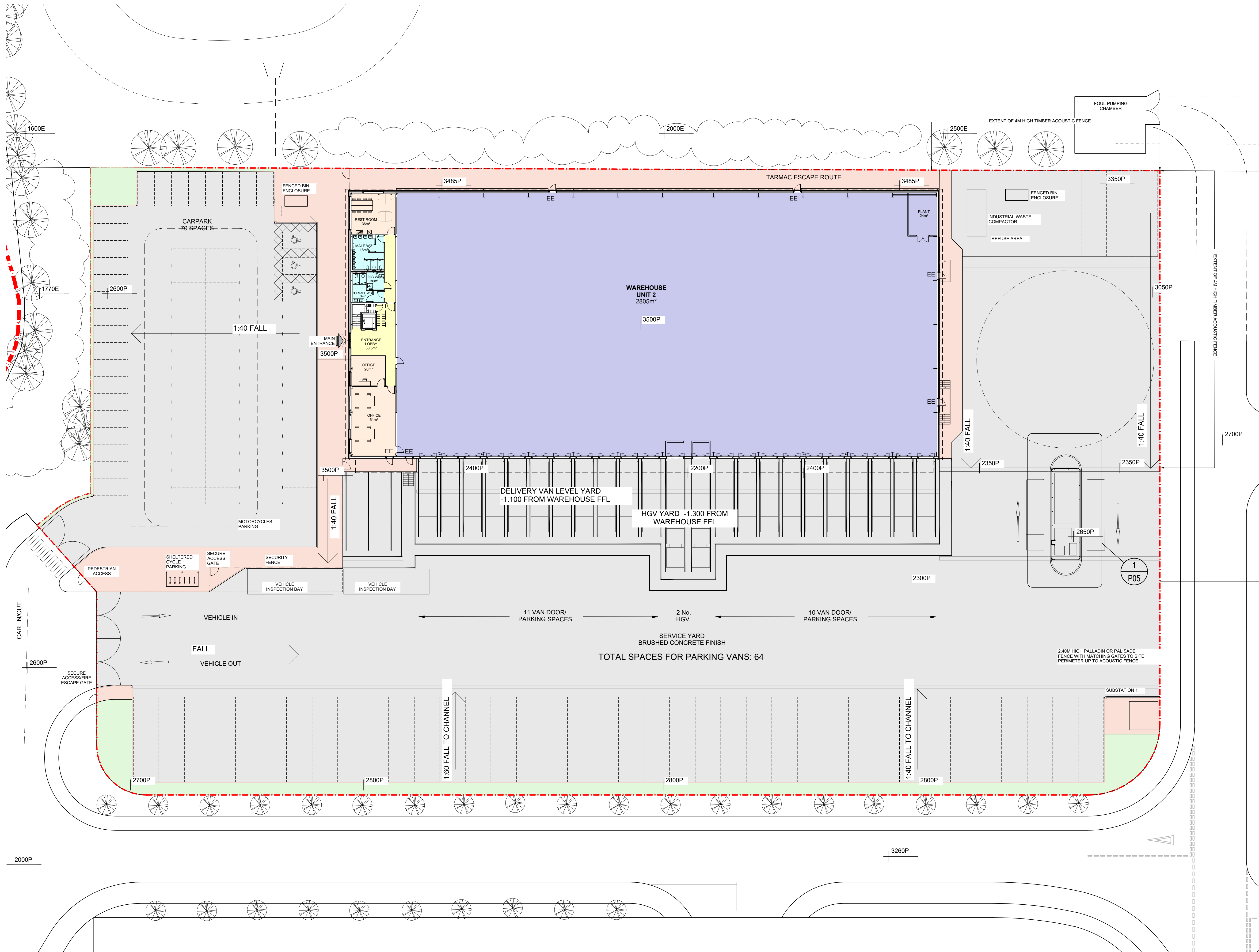
1 PROPOSED GROUND FLOOR PLAN 1 : 250
