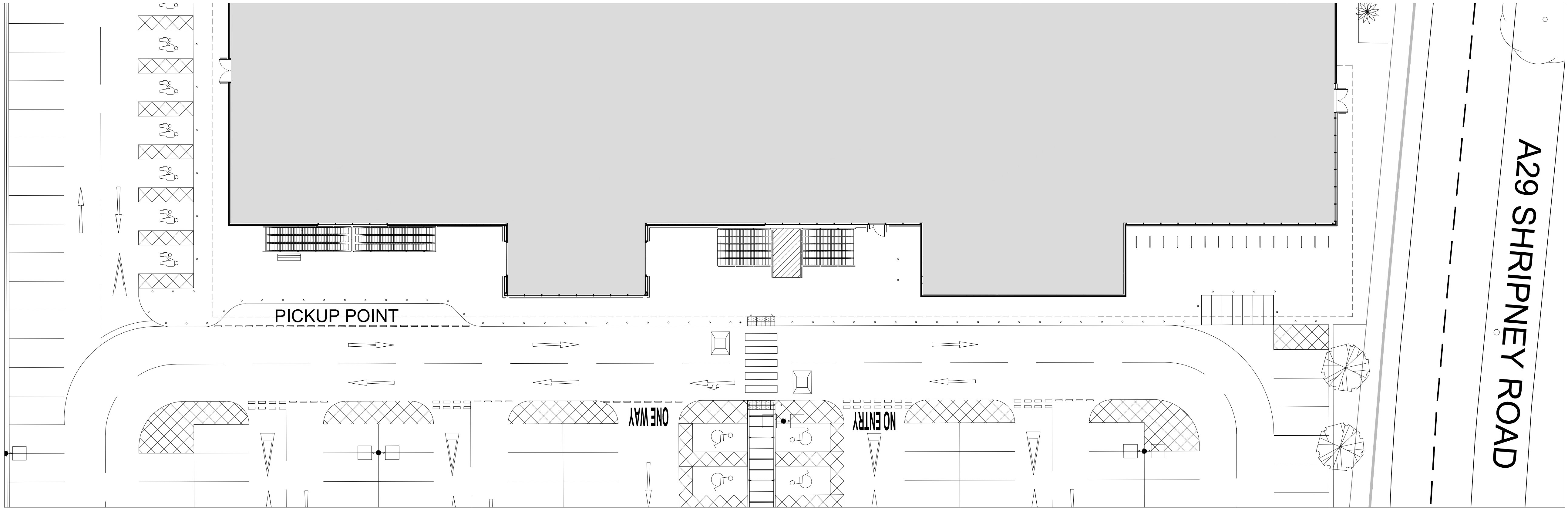
Existing Detail Site Plan
