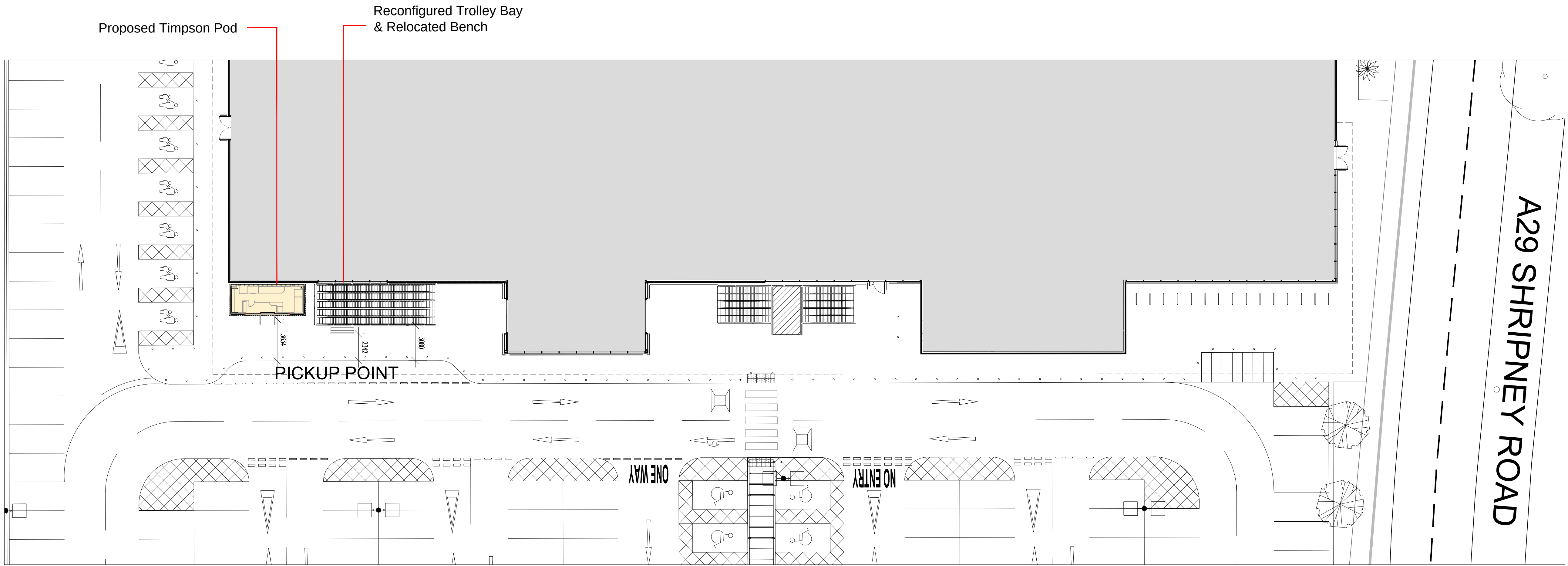
Proposed Detail Site Plan
