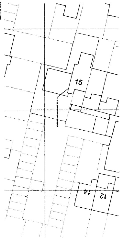
BLOCK PLAN 1:200
