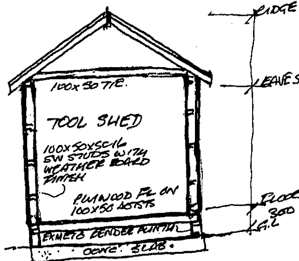
SECTION
