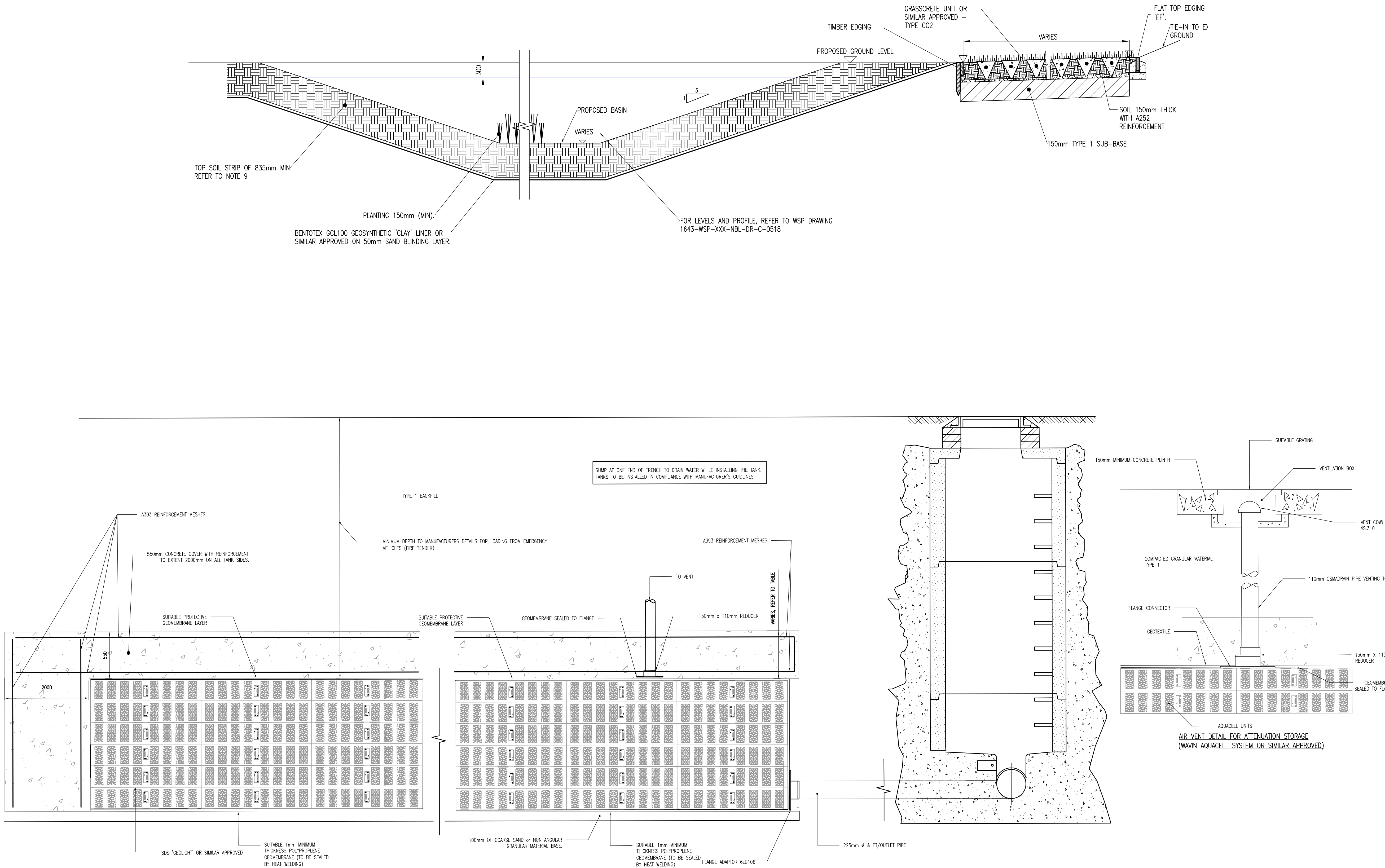
TYPICAL ARRANGMENT OF ATTENUATION STORAGE (CELLULAR STRUCTURE)
