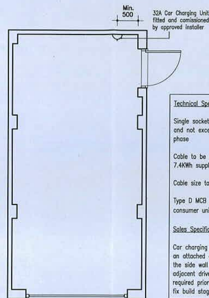
Indicative Floor Plan.
