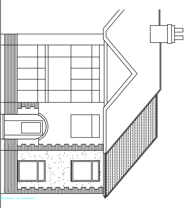
Proposed Front Elevation (South)
