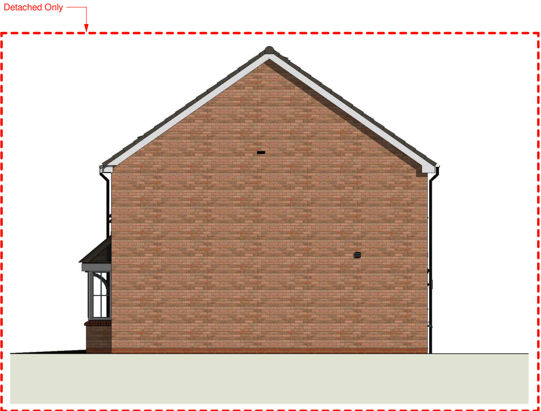
4 Gable Elevation 1 : 100
