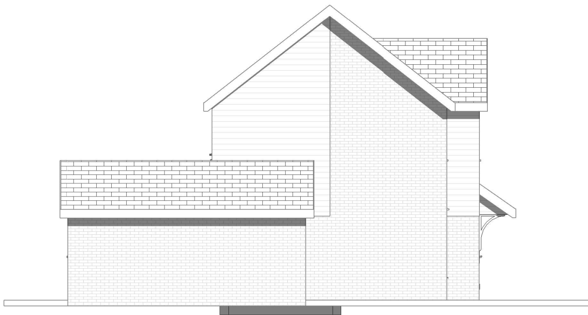
Proposed Elevation Left side WEST
