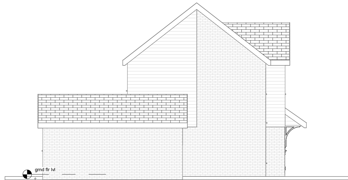
Existing Elevation Left side WEST
