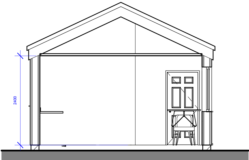
1 | Building Section 1 : 50
