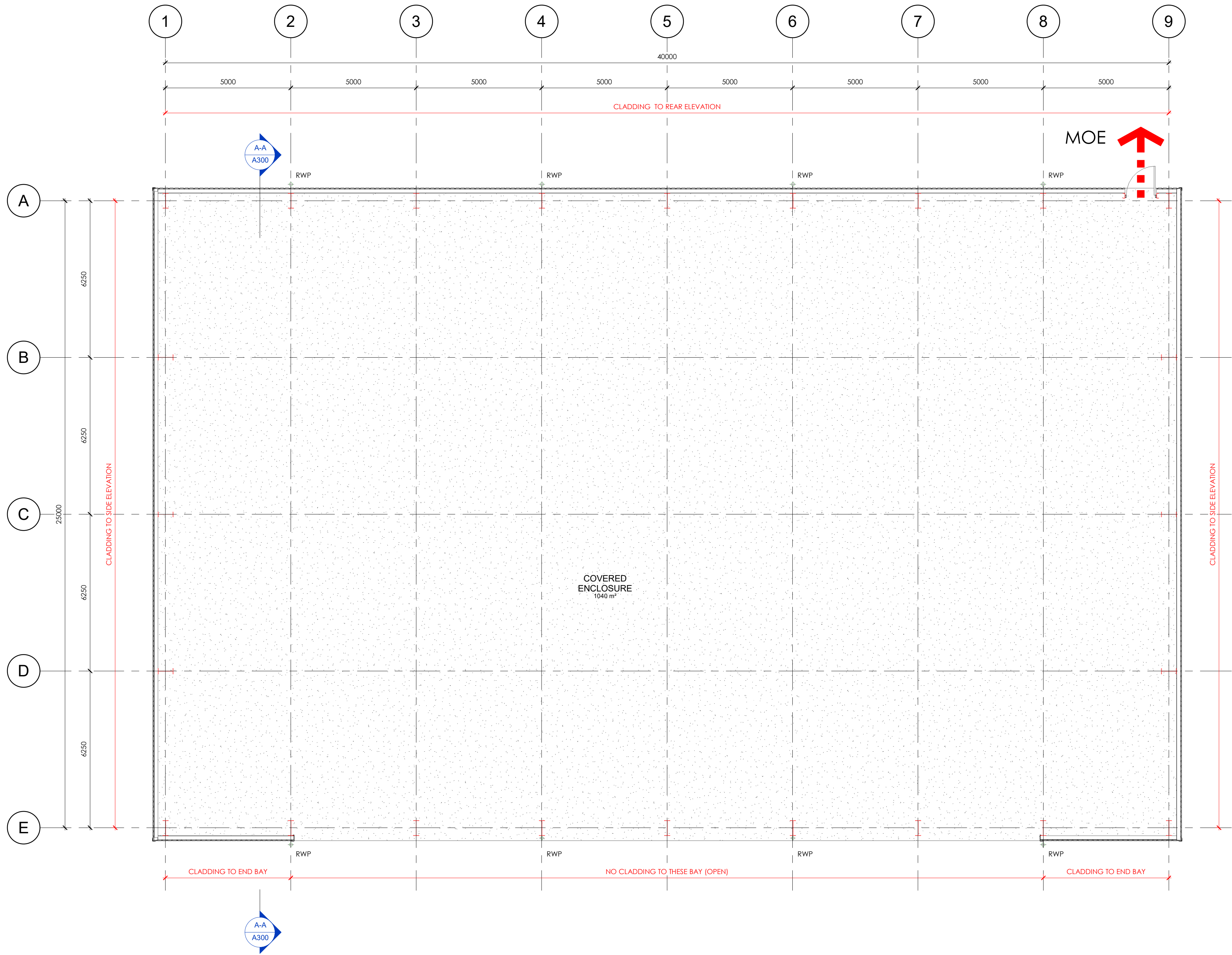
GROUND FLOOR GA PLAN 1 : 100
