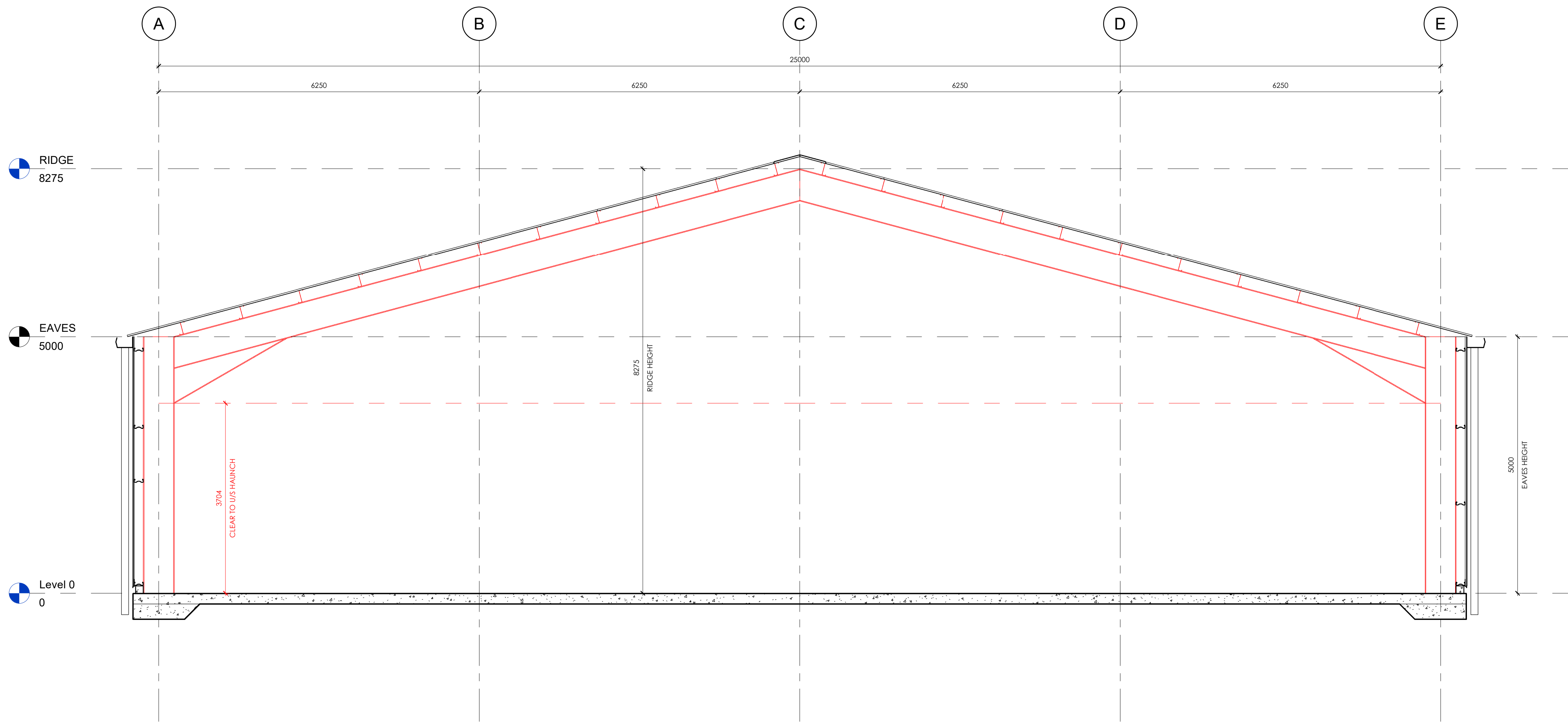
TYPICAL SECTION A-A 1 : 50
