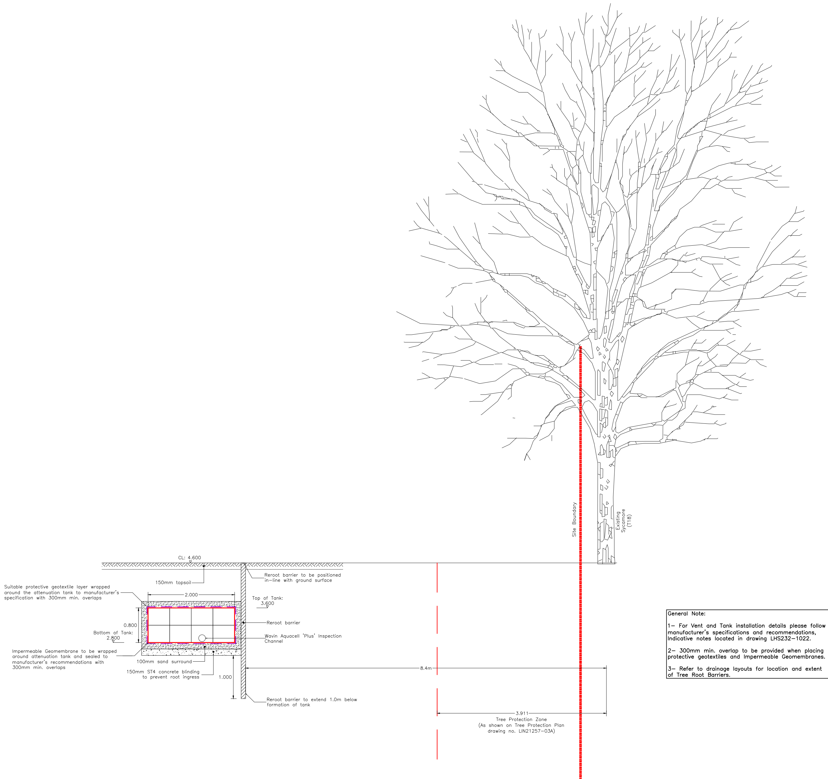
Reroot Barrier Detail Scale 1:50
