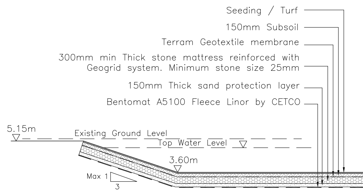
TYPICAL POND SECTION Scale 1:100
