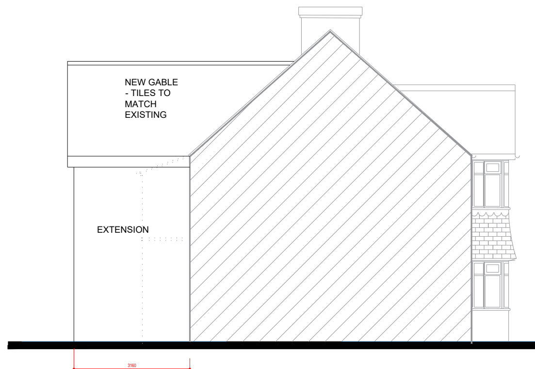
EAST (SIDE) ELEVATION PROPOSED
