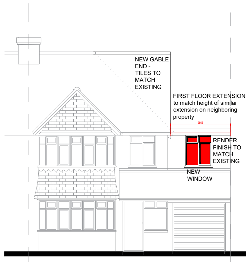
NORTH (FRONT) ELEVATION PROPOSED
