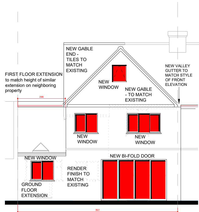
SOUTH (REAR) ELEVATION PROPOSED
