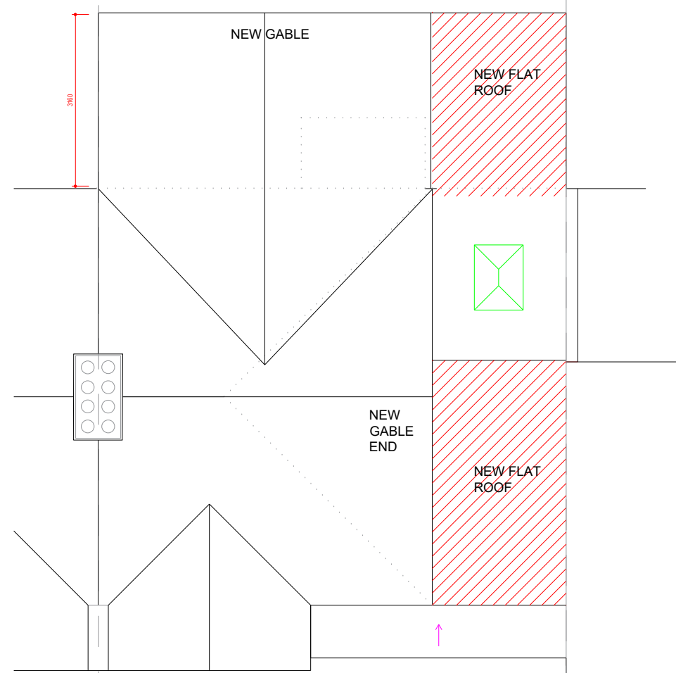
ROOF PLAN - PROPOSED
