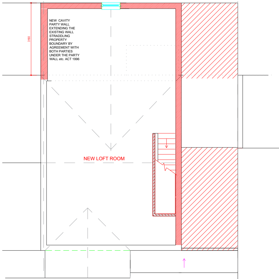
LOFT - PROPOSED
