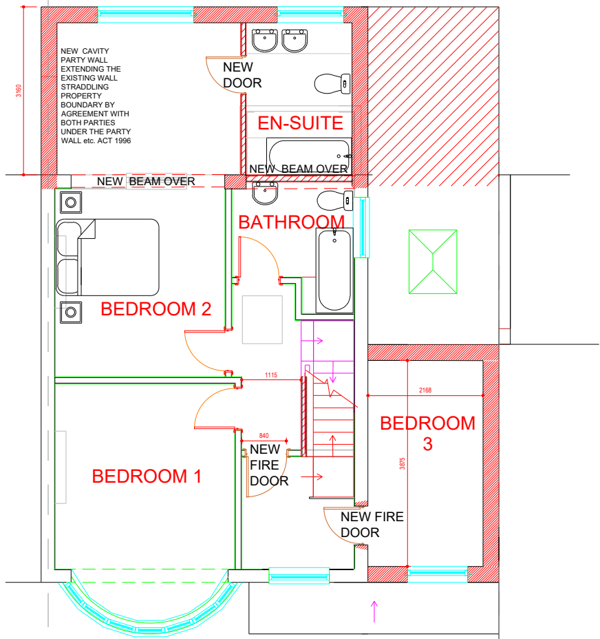
FIRST FLOOR - PROPOSED
