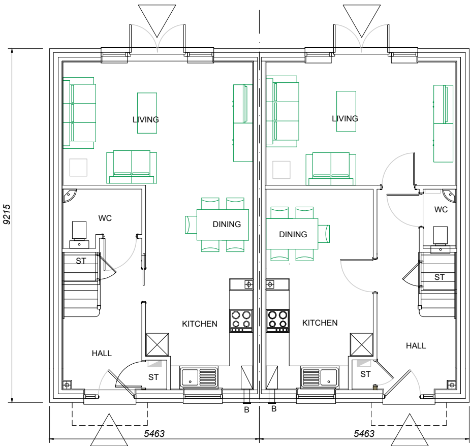
Plot 73 303 Plot 74 303A GROUND FLOOR PLAN
