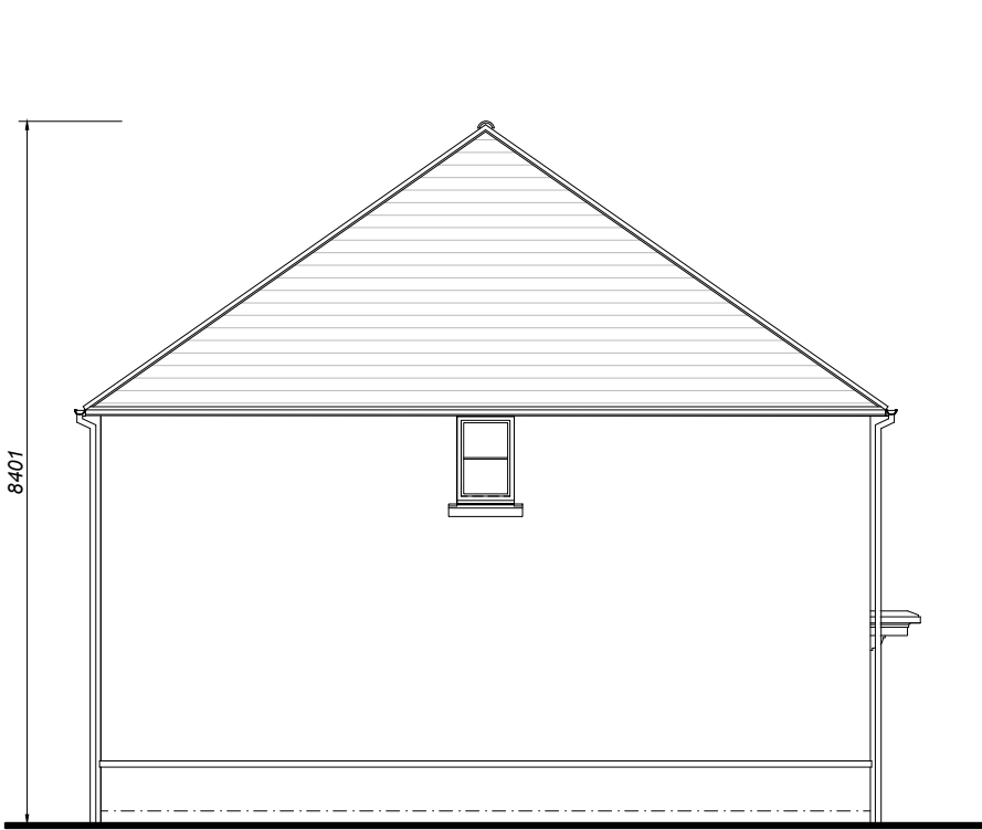
Plot 73 303A SIDE ELEVATION
