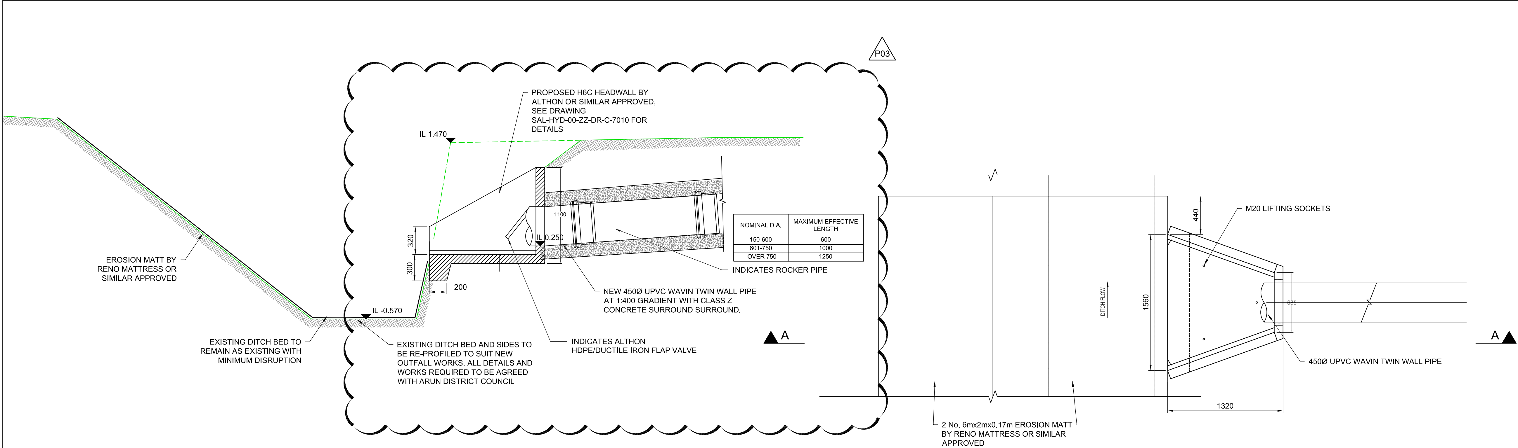
SECTION A-A SEE DRAWING SBX-KSA-Z0-XX-DR-C-6800 FOR PLAN
