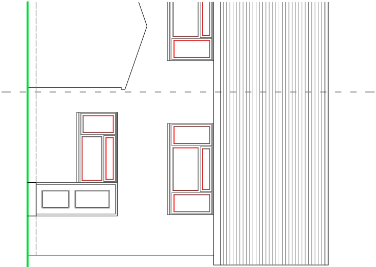
REAR ELEVATION
