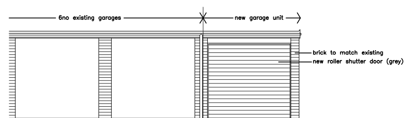
Front elevation
