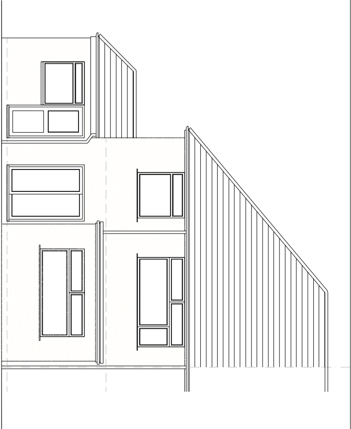
Rear Elevation
