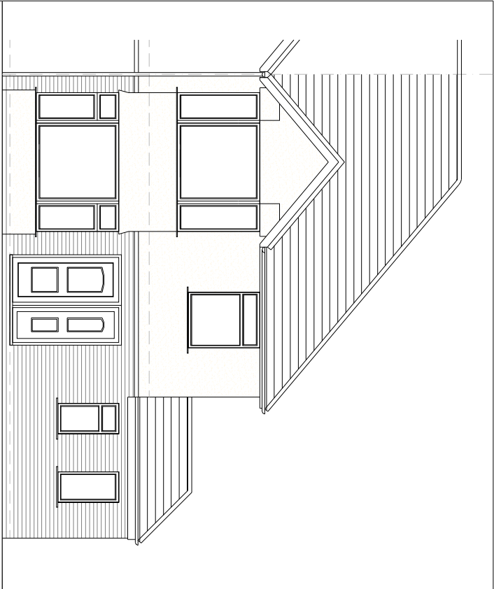
Front Elevation
