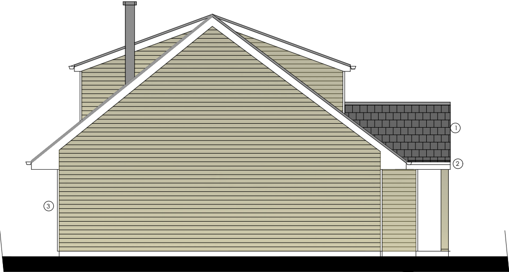
Side Elevation
