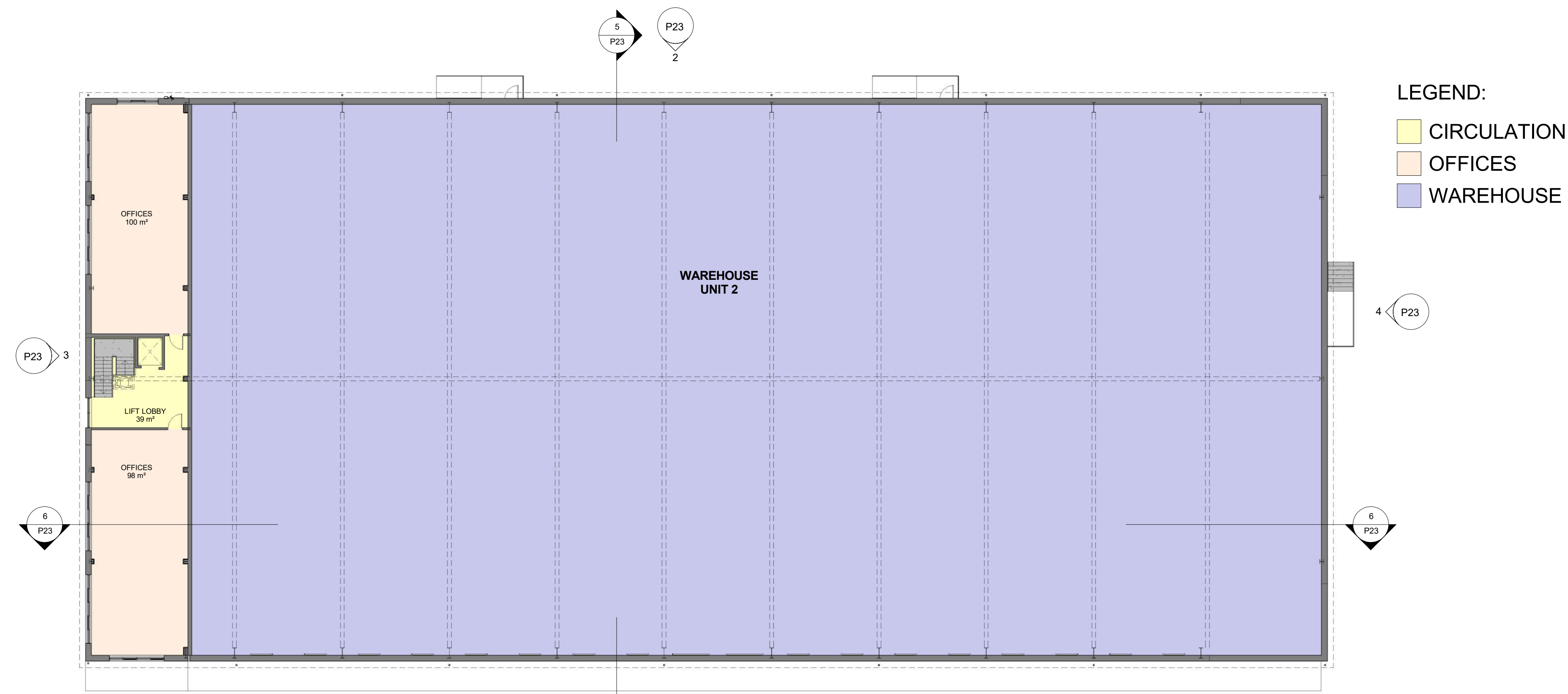
1 FIRST FLOOR - OFFICE 1 : 200
