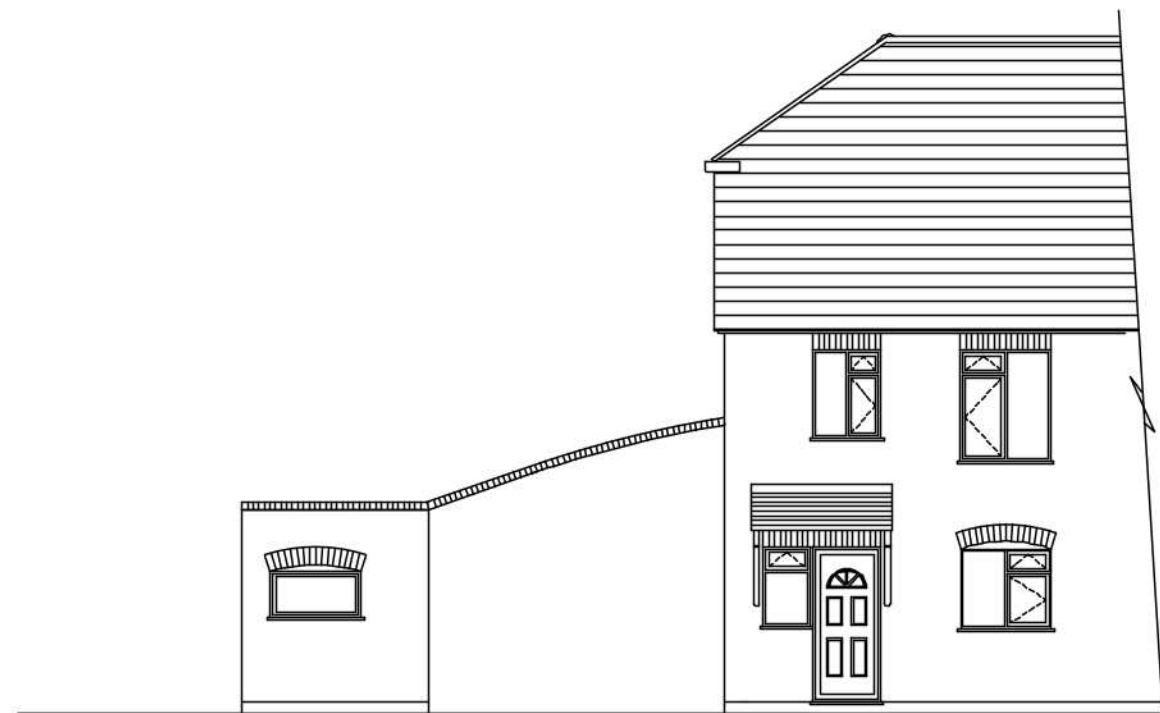
Existing NNW Elevation
