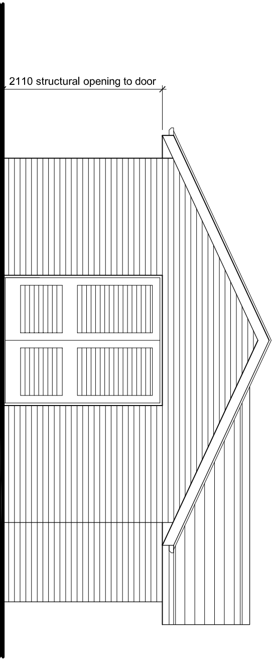
EAST ELEVATION (Bin store entrance)
