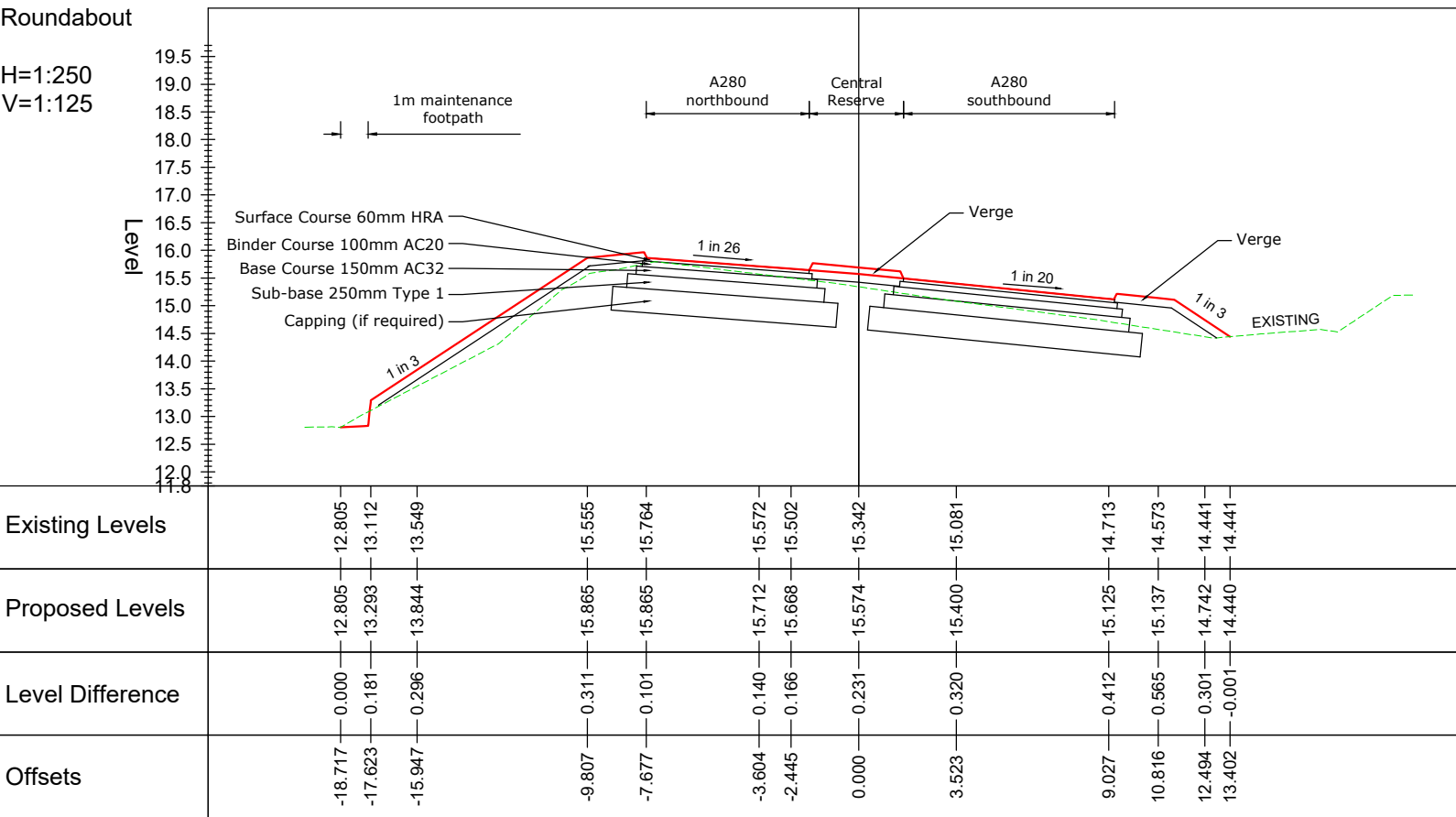
SECTION B - B A280 Typical Cross Section
