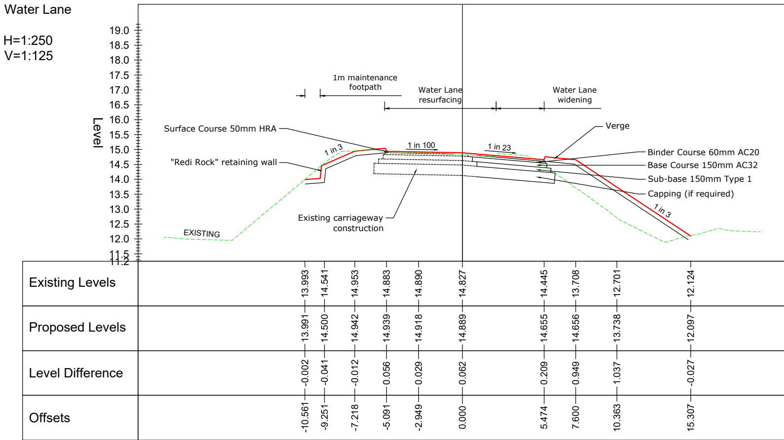
SECTION A - A Water Lane Typical Cross Section
