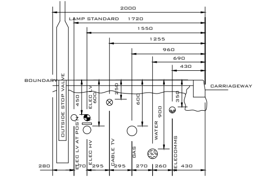
NJUG RECOMMENDED ARRANGEMENT OF MAINS IN A FOOTWAY, INCLUDING CABLE TV DUCTS 1:50 SCALE @ A1
