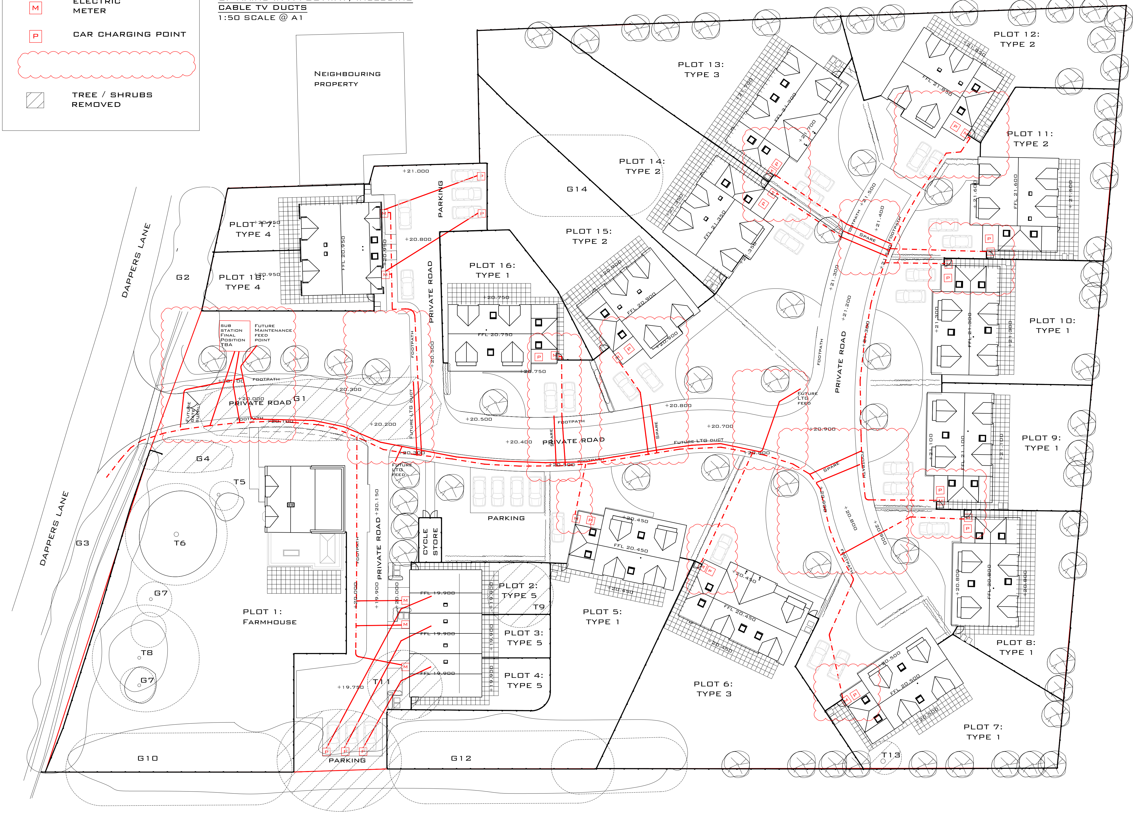
PROPOSED INCOMING ELECTRIC SERVICES PLAN 1:250 SCALE @ A1
