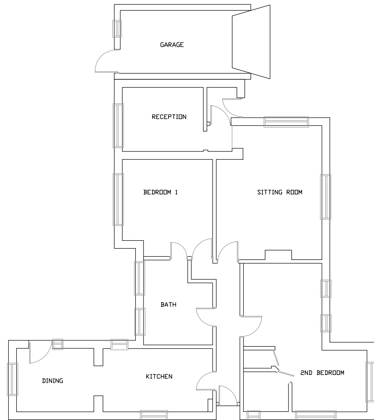
EXISTING FLOOR PLANS 1:100
