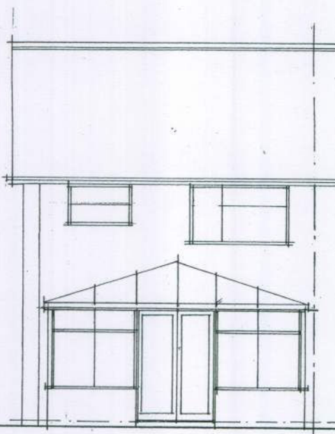
WEST 1/100
