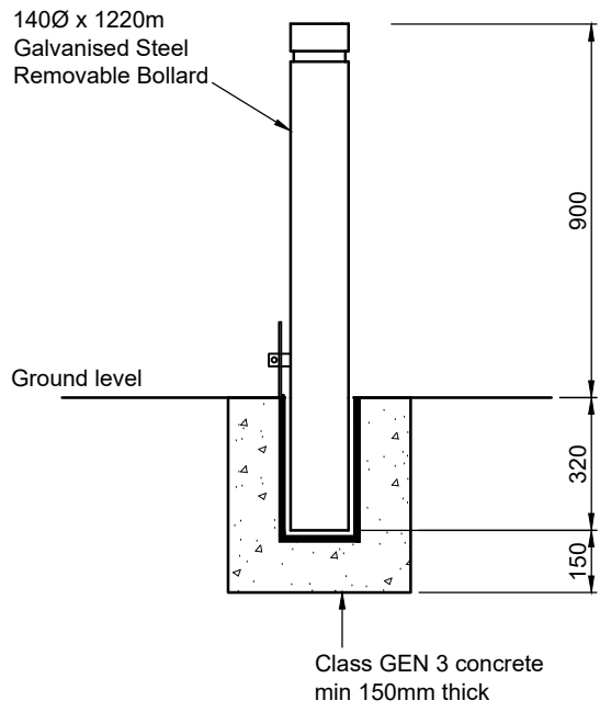
REMOVABLE BOLLARD DETAIL (Scale 1:20)
