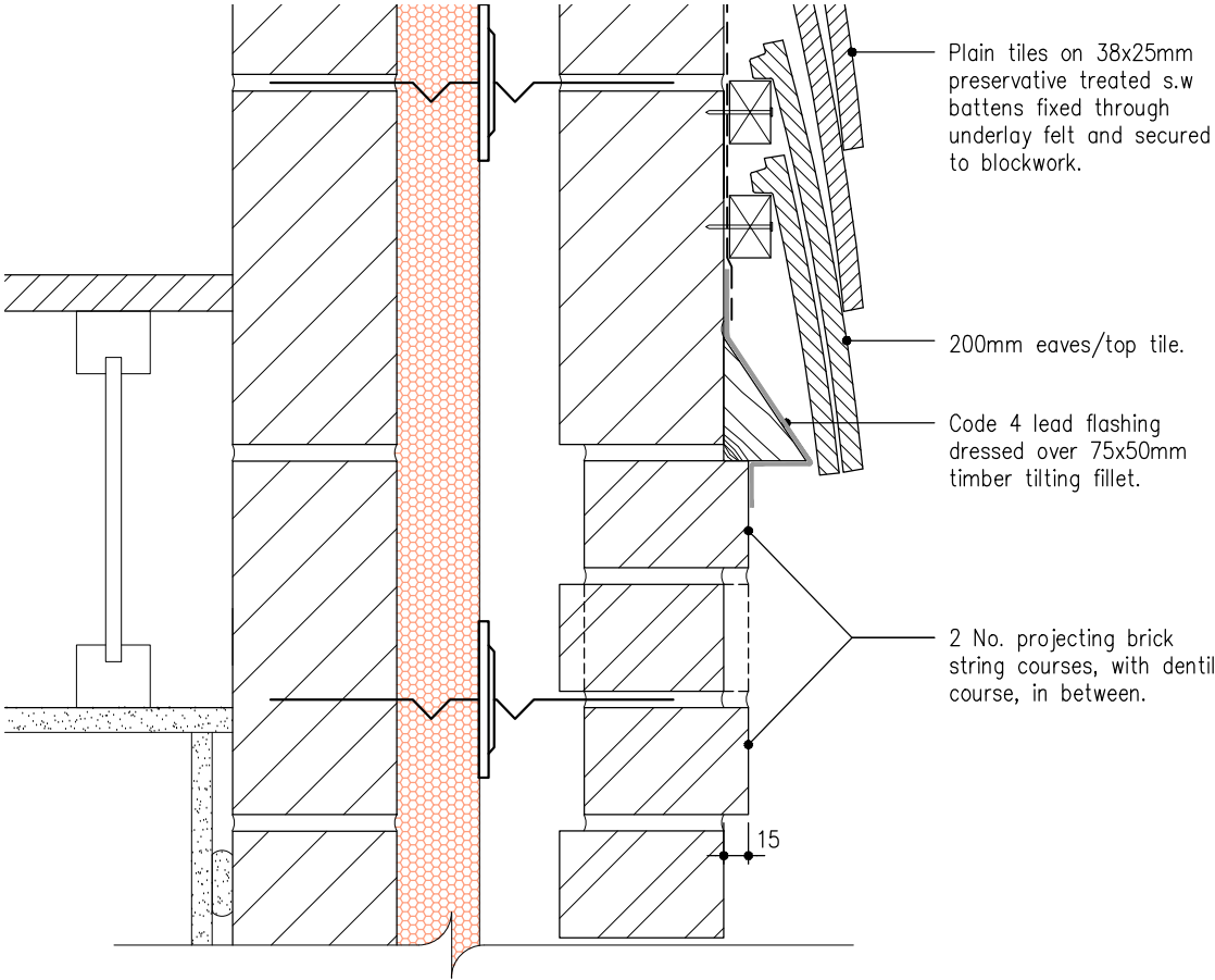
Bottom Termination/Junction With Brickwork
