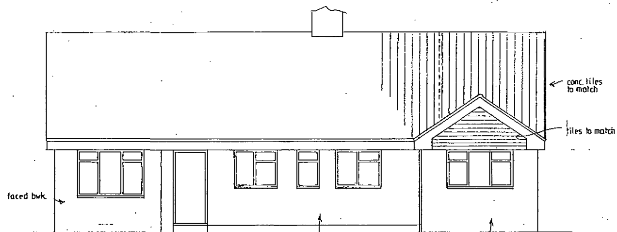
FRONT [NORTH] ELEVATION
