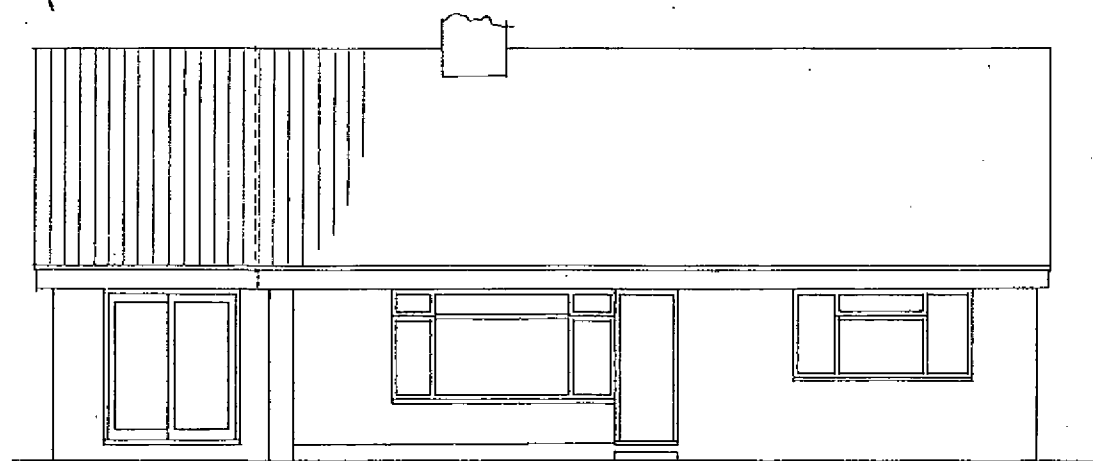
REAR [SOUTH] ELEVATION
