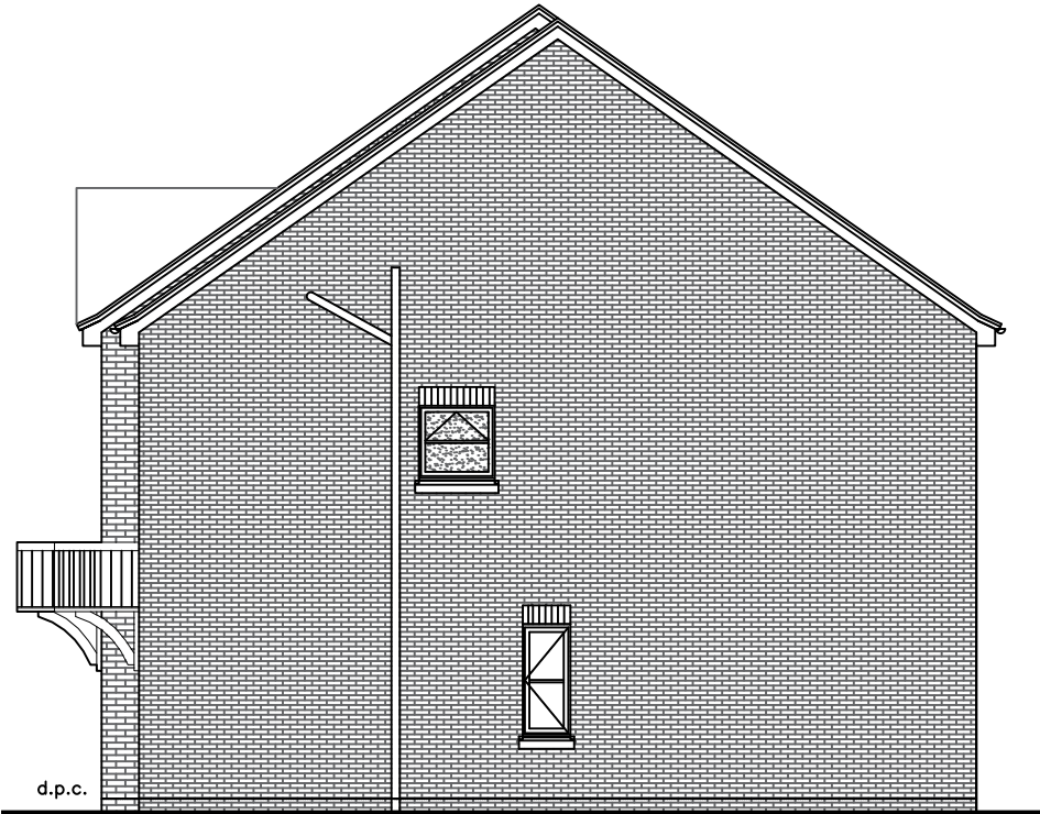
Side Elevation
