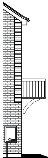
Side Elevation (weatherboarding)
