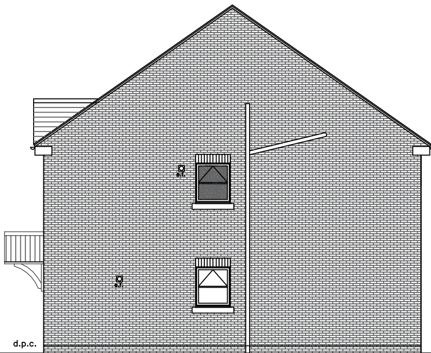
Side Elevation
