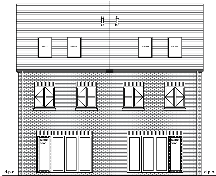
Rear Elevation
