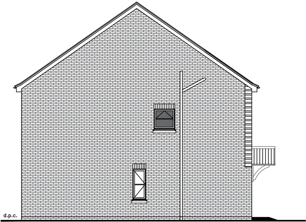
Side Elevation (Plot 17)
