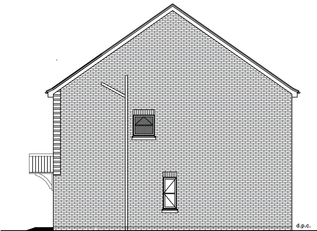
Side Elevation (Plot 16)
