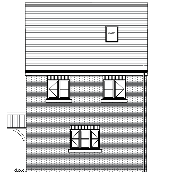
Side Elevation
