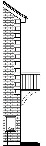
Side Elevation (hanging tile)
