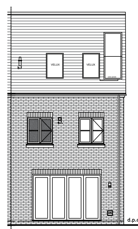
Rear Elevation
