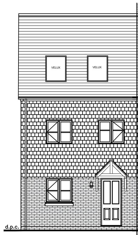
Front Elevation (hanging tile)
