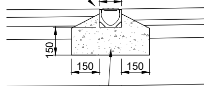
ACO CHANNEL DRAIN DETAIL (Scale 1:20)
