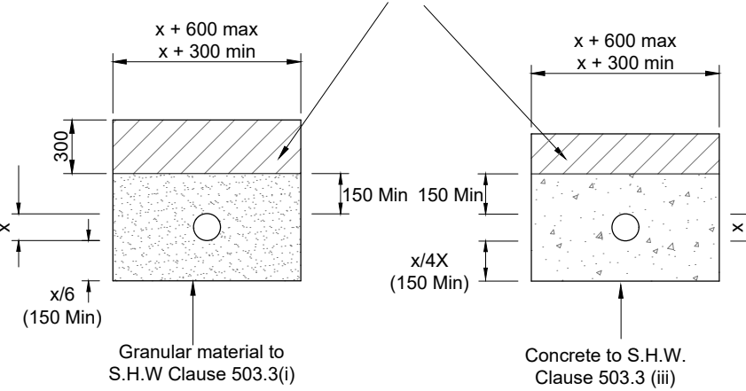
CLASS S PIPE BEDDING
