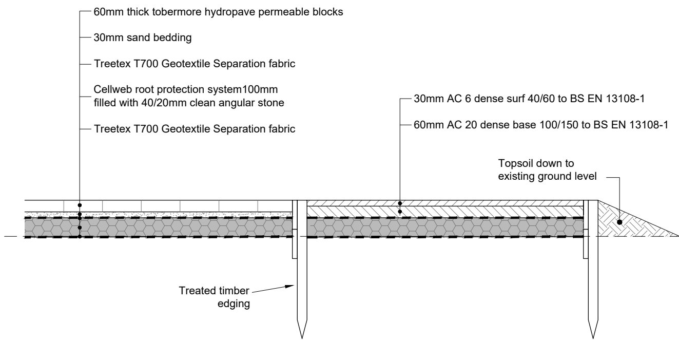
PV3 - NO DIG CONSTRUCTION (Scale 1:20)
