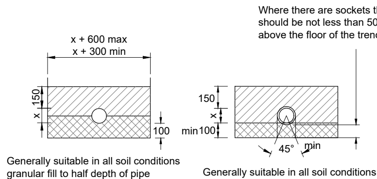
CLASS B PIPE BEDDING
