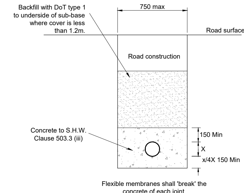
PIPE BEDDING FOR ADOPTABLE DRAINS UNDER HIGHWAY CONSTRUCTION
