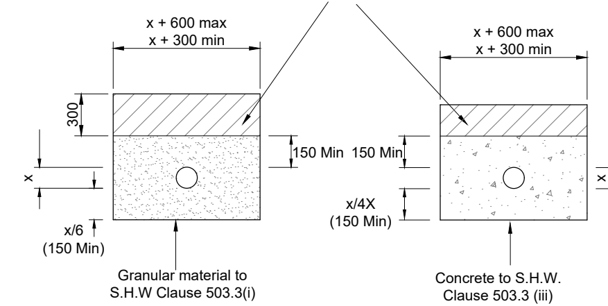
CLASS S PIPE BEDDING
