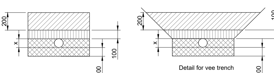
PIPE BEDDING FOR FLEXIBLE PIPES
