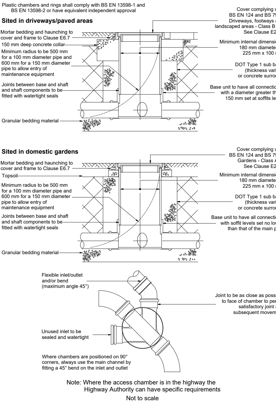
FIGURE B.21 TYPICAL INSPECTION CHAMBER DETAIL - TYPE 4 (Flexible material detail) Maximum depth from cover level to soffit of pipe 2 m, non-entry
