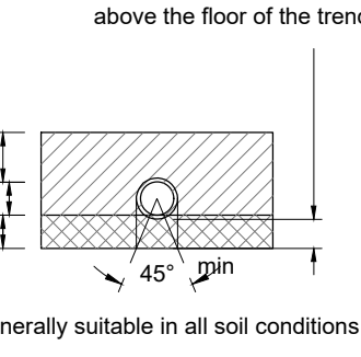
CLASS F PIPE BEDDING
