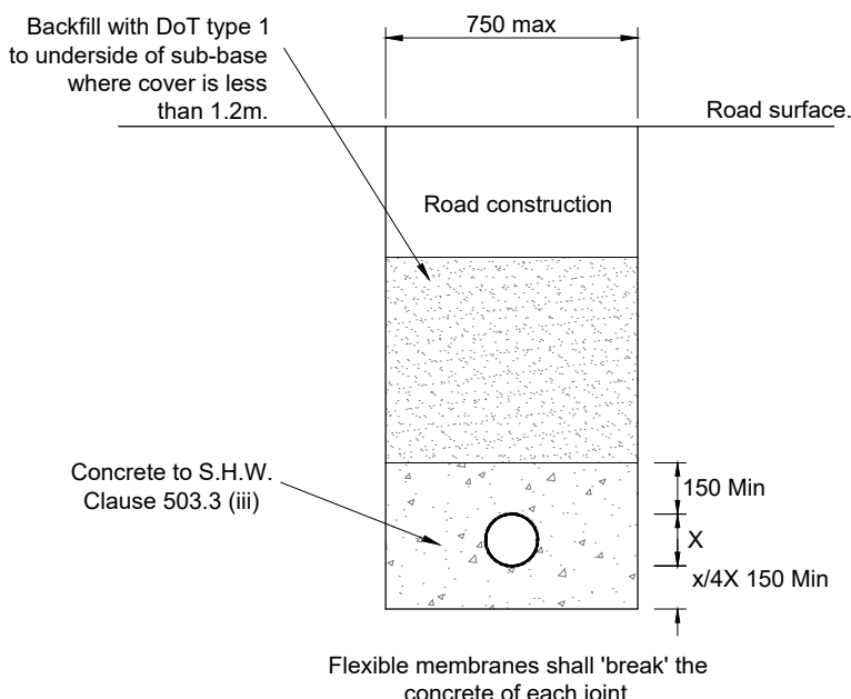
PIPE BEDDING FOR ADOPTABLE DRAINS UNDER HIGHWAY CONSTRUCTION
