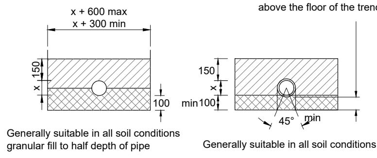
CLASS B PIPE BEDDING
