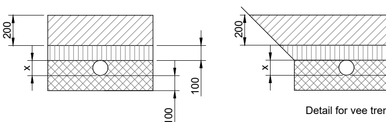
PIPE BEDDING FOR FLEXIBLE PIPES
