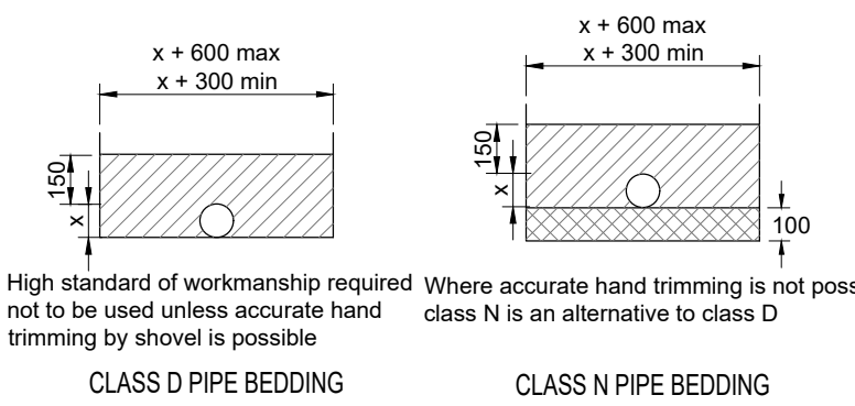
CLASS D PIPE BEDDING
