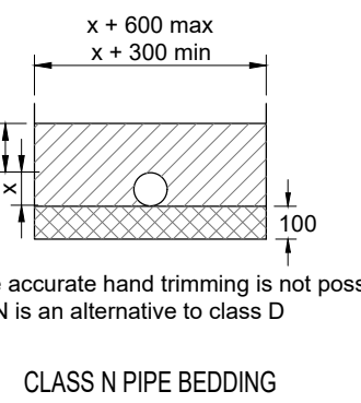
CLASS N PIPE BEDDING
