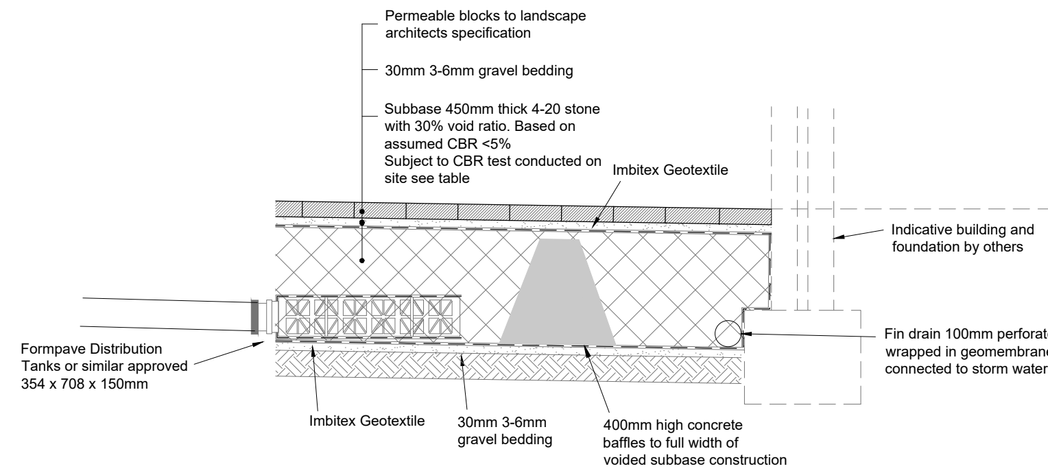
BLOCK CARRIAGEWAY AND DRIVES VOIDED SUBBASE INFILTRATION SYSTEM (Scale 1:20)
