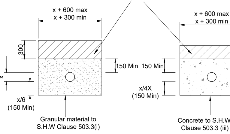
CLASS S PIPE BEDDING
