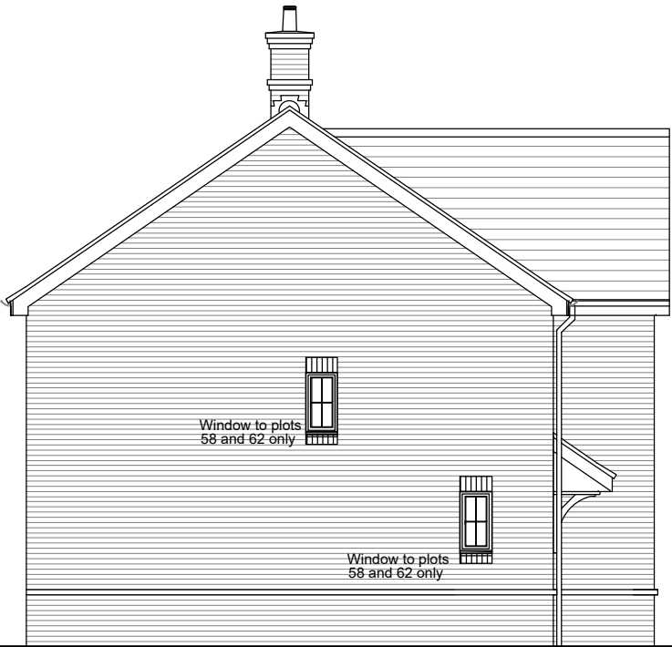
Side Elevation
