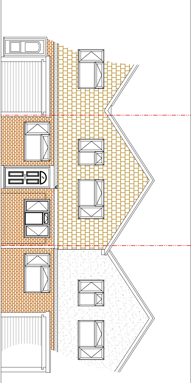
No. 45 No. 43 No. 41 NORTH ELEVATIONS
