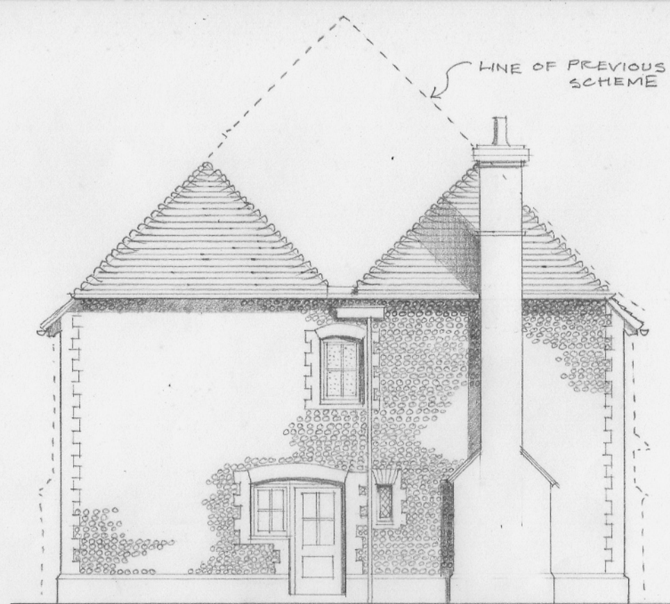
UNIT 2: PROPOSED WEST ELEVATION SCALE 1:100.
