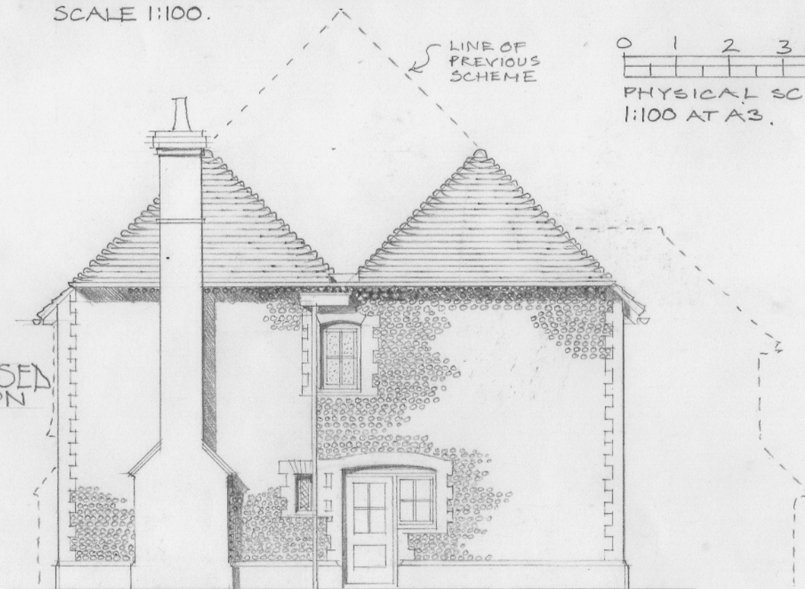
UNIT 1: PROPOSED EAST ELEVATION SCALE 1:100.
