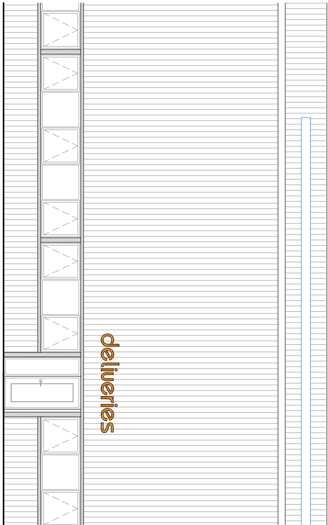
+EL Proposed partial (south) elevation - scale 1:100 at A1 Scale in Metres 0 1 2 3 4 5 10
