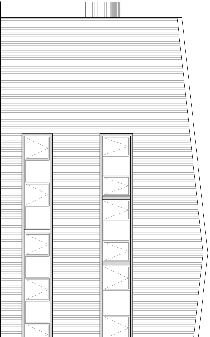
+EL Proposed partial (east) elevation - scale 1:100 at A1 Scale in Metres 0 1 2 3 4 5 10
