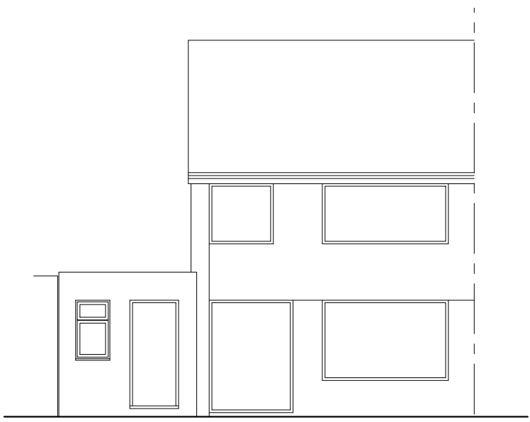
Pr. East elevation (front) 1:100 @ A3
