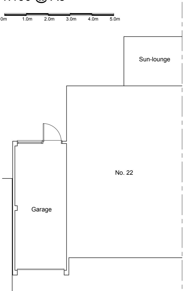
Ex. Ground floor plan 1:100 @ A3
