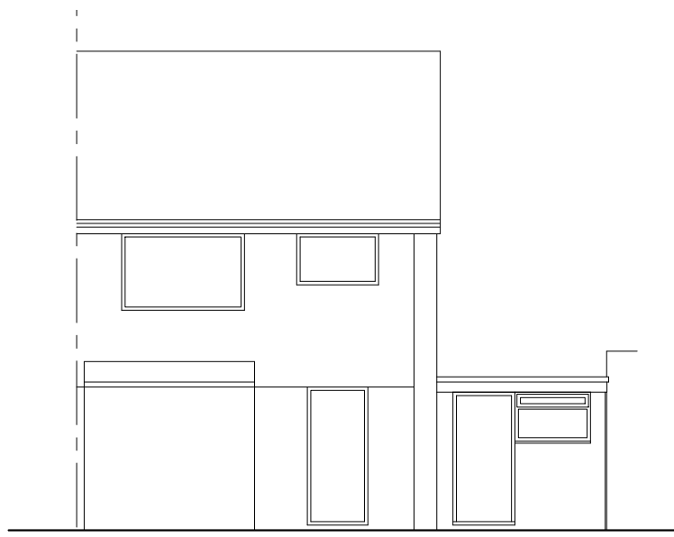
Ex. West elevation (rear) 1:100 @ A3
