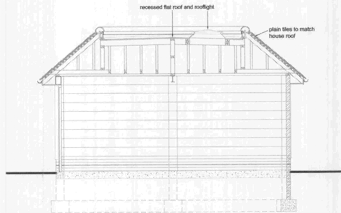
1:50 GARAGE SECTION B-B
