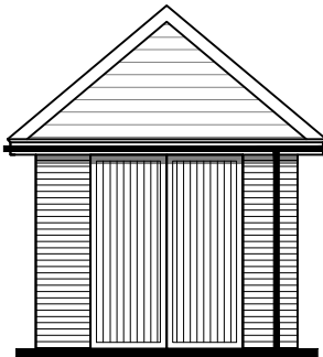
Proposed Front Elevation
