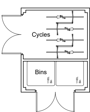
Proposed Bin and Cycle Store Plan Plots 29-32
